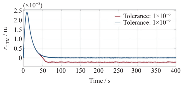
图 6 不同容差 \varepsilon 和 \epsilon 下检验质量捕获量测信号的对比 Fig. 6 Comparison of test mass capture measurement signals with different tolerances \varepsilon and \epsilon
