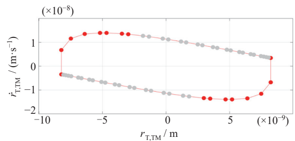
图 8 最小鲁棒正不变集修正 Fig. 8 Correction of minimum robust positive invariant set
