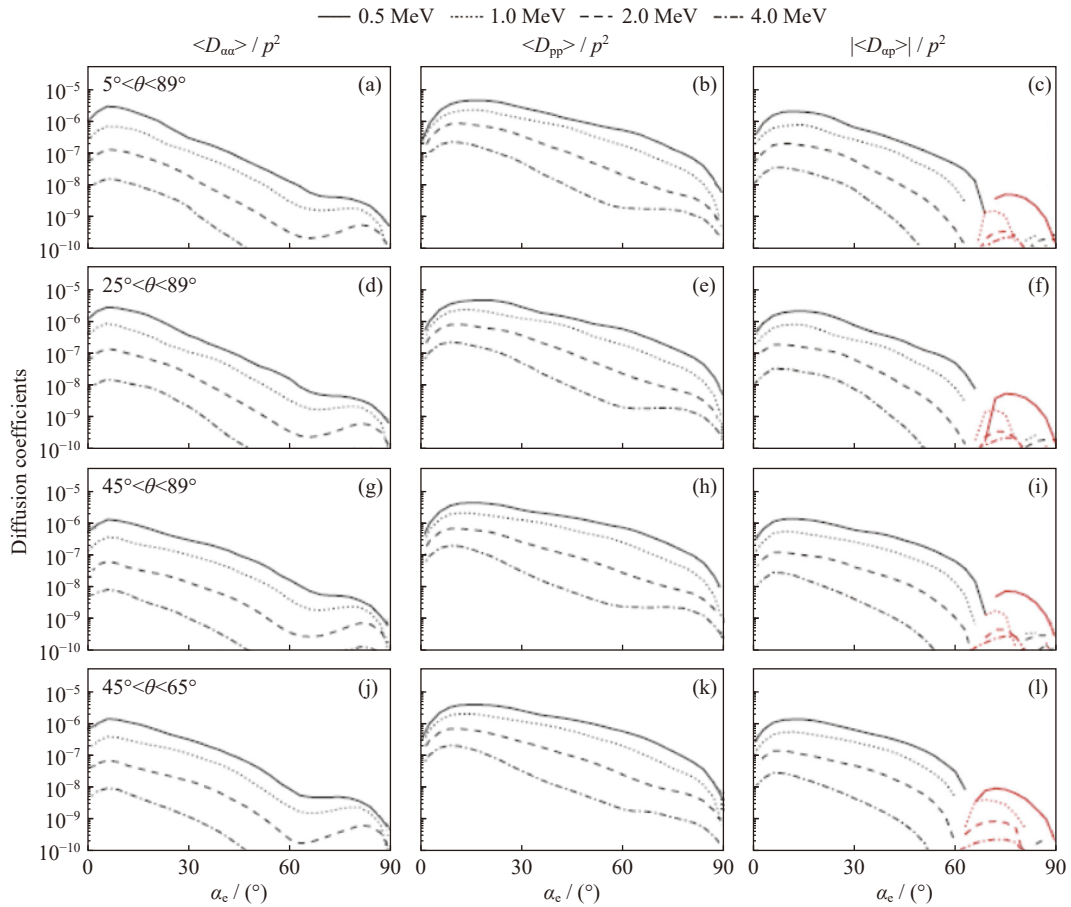
图 5 不同传播角分布的投掷角(左)、动量(中)及投掷角-动量交叉(右)弹跳平均扩散系数 1D 结果 Fig. 5 1D bounce-averaged diffusion coefficients of pitch angle (left), momentum (middle), and cross (right) for different wave normal angle distributions
